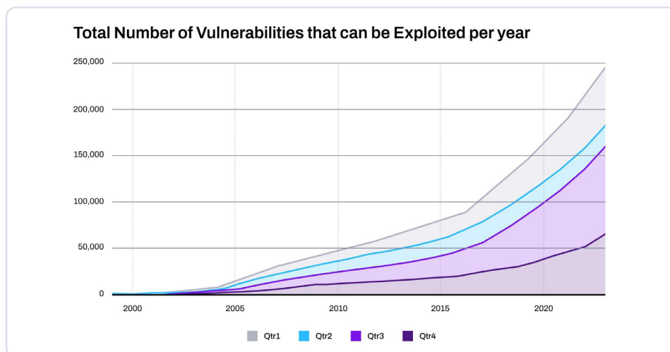
Figure 1: The graph highlights the hockey stick-like growth of vulnerabilities. The breakneck increase in vulnerabilities is so bad that NVD, the official repository for the world, can't keep up.
