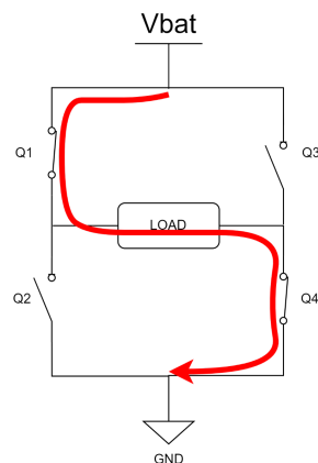
State 1 - V_{bat} load voltage
