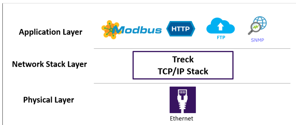
Network attack-surface of an NMC
